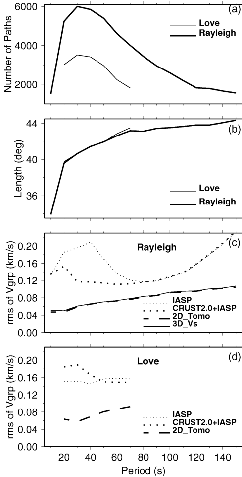
Fig. 4. Statistics of the data used in this study: (a) number of paths for each period of Rayleigh waves (thick line) and Love waves (thin line); (b) average path length, in degrees, of all paths for each period and wave type; (c) Rayleigh wave group-velocity deviations from the IASP model, the initial CRUST2.0 + IASP model, the 2D tomographic model, and the inverted 3D S-velocity model; (d) the same as (c), but for Love wave.
