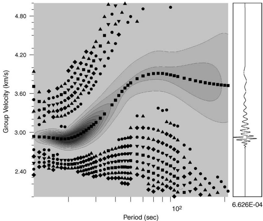
Fig. 3. An example of Rayleigh-wave dispersion processing with Multiple Filtering Technique (MFT). The left shows the amplitude spectrum of the multiple filtered seismogram. The right shows the phase-matched filtered seismogram used in the MFT. For each period, the black square in the center of the darkest contour is the maximum energy and represents a point in group-velocity dispersion. Other symbols are secondary peaks.
