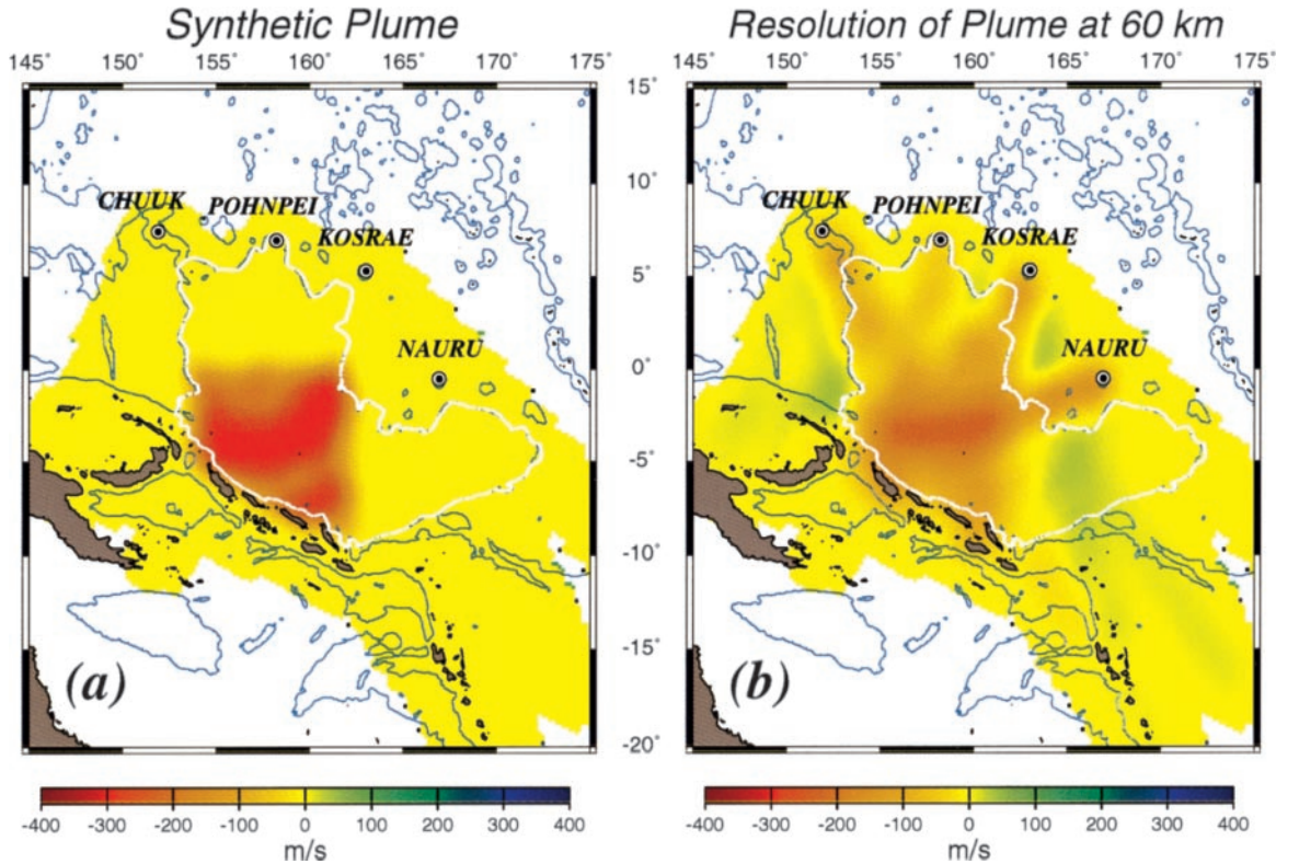
Fig. 5. Test of the resolution of a synthetic ‘‘plume’’ conceptually similar to the structure detected under the OJP. (a) Map view of the input model (at 60 km depth). (b, c and d) Same as Fig. 4c–e for the inversion of the plume model. (e and f) Same as (c) and (d) for a plume composed of depth layers alternatively fast and slow. Note the practical absence of vertical smearing.
